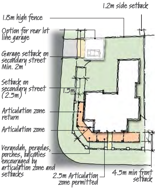
FIGURE 22: Example of Corner Lot Articulation Zone
