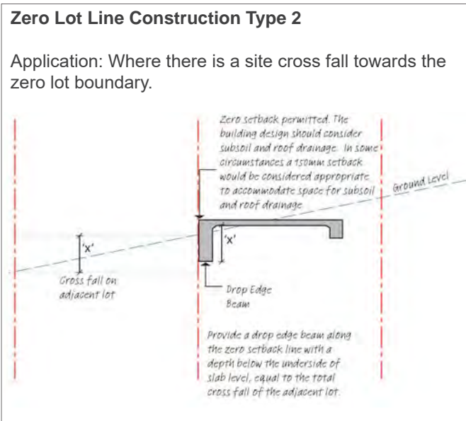
FIGURE 16: Zero Lot Line Construction Type 2
