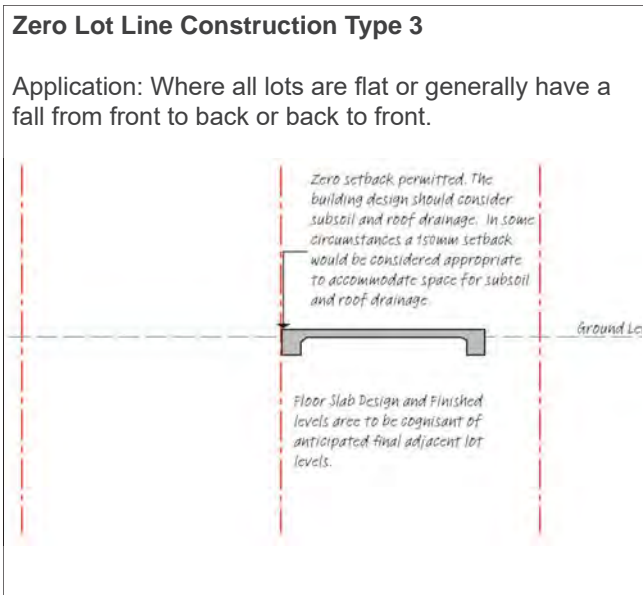
FIGURE 17: Zero Lot Line Construction Type 3
