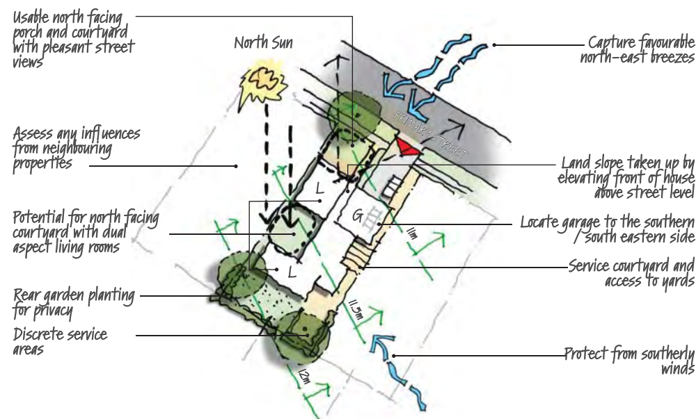
FIGURE 5: Example of site analysis diagram
