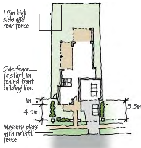
FIGURE 30: Side and rear fencing (with front fence type 1)
