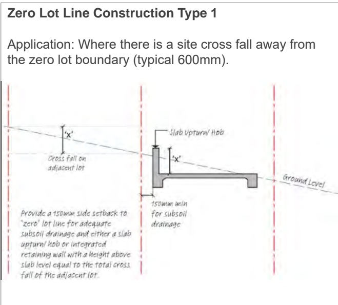
FIGURE 15: Zero Lot Line Construction Type 1
