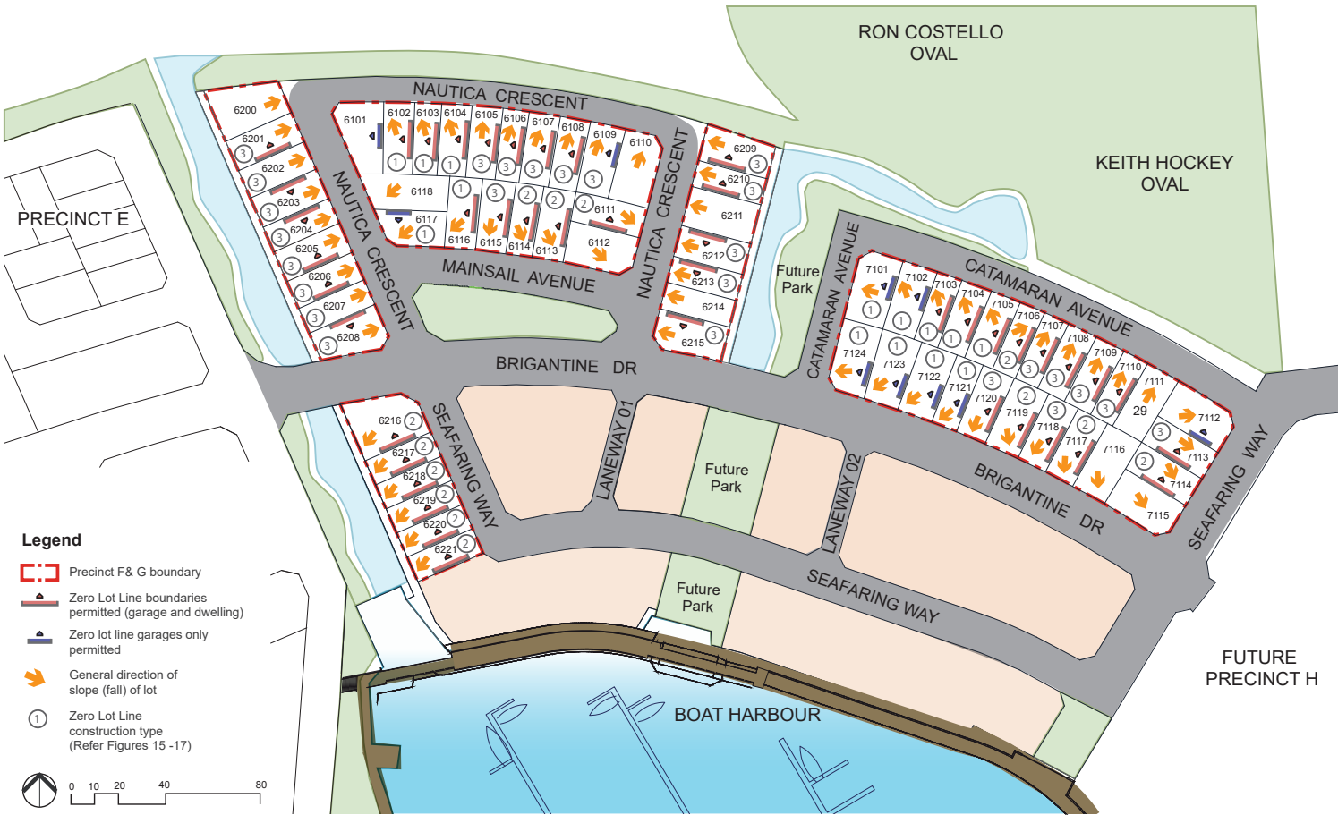
FIGURE 13: Zero Lot Line Building
