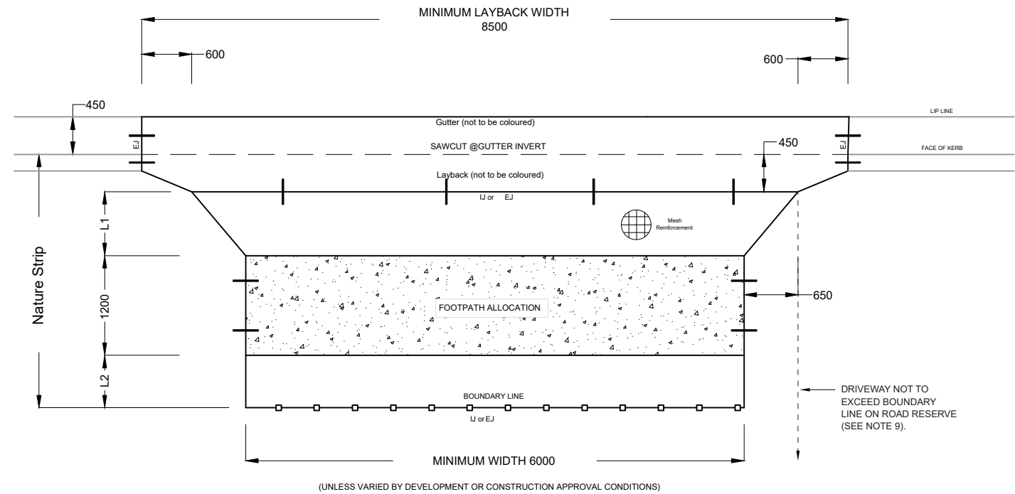
STANDARD INDUSTRIAL DRIVEWAY AND FOOTPATH CROSSINGS OPTION 1
