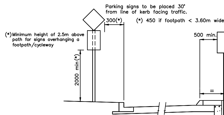
URBAN ROADS
