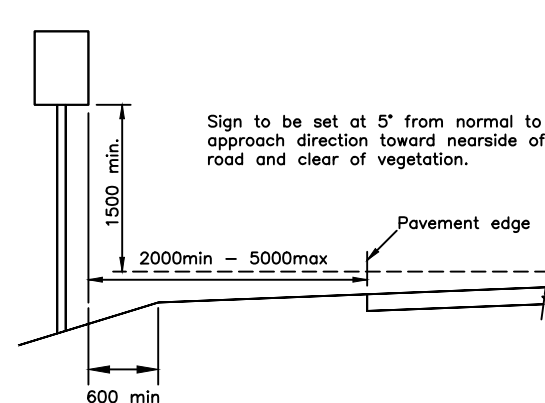
RURAL ROADS
